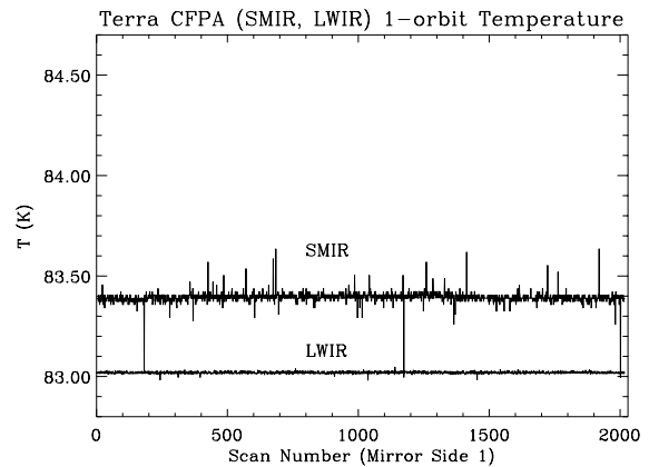
Fig. 10. Terra MODIS SMIR and LWIR temperatures (same date/time as in Fig. 9).
